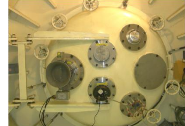
CABIN PRESSURE RIG
